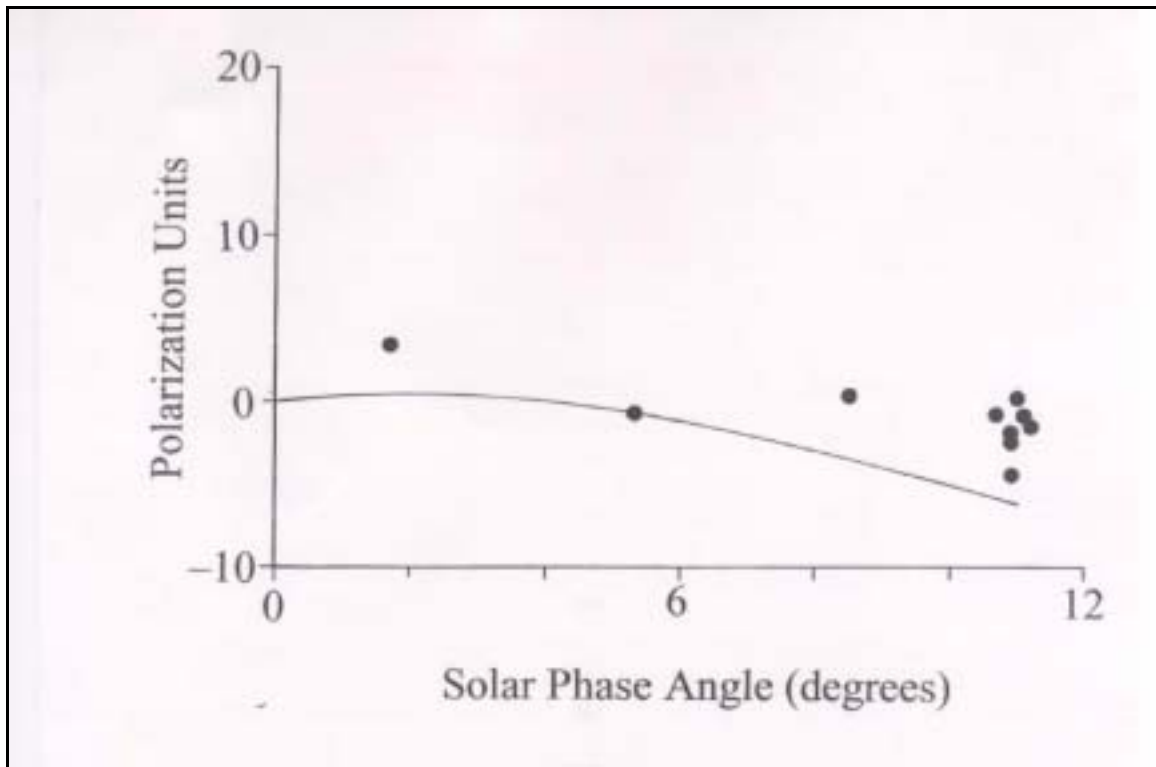
Figure 10: Amount of polarized light reflected by Jupiter as a function of the solar phase angle during the 2001-02 apparition shown as dots. All measurements were done in the V filter. The curve is based on Lyot's measurements made between 1923 and 1926 (Dollfus, 1961, 392).
