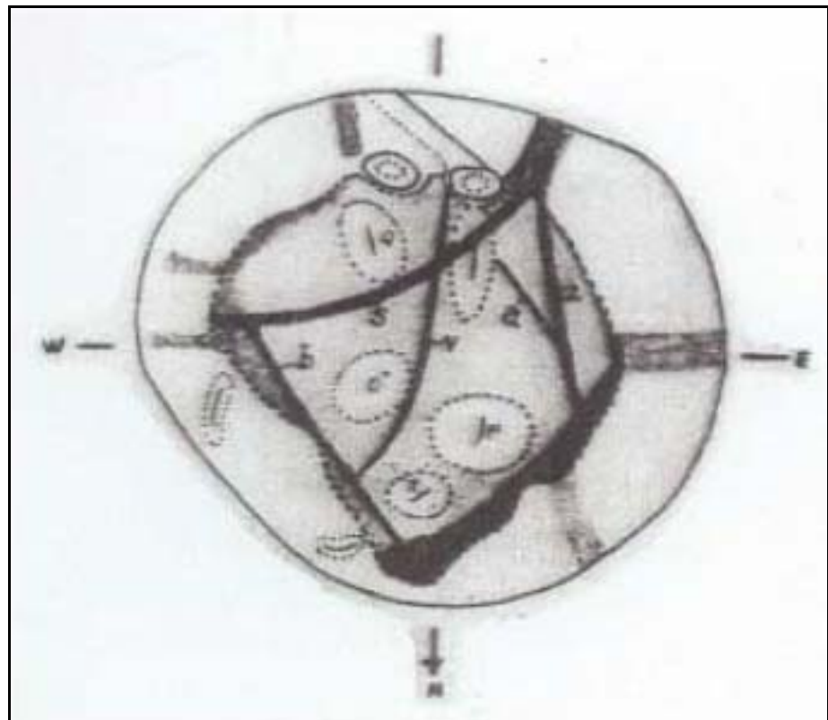
Figure 5. Map of Lunar Crater Conon by Elmer J. Reese. Based upon many observations by himself and others, chiefly in 1947-49.
