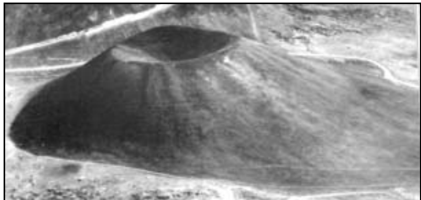
Figure 4: A volcanic cinder cone in Hawaii. (From Carr and Greeley, Volcanic Features of Hawaii , p. 37.
