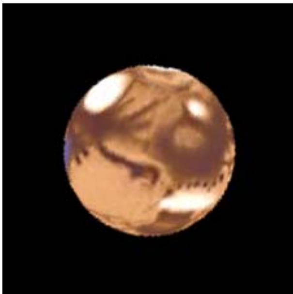
Figure 1: Color version of the 2000-2001 Mars apparition map. South is at top. The white seen over the South Polar Region during most of the observing season is the South Polar Cap. North is at bottom and shows the bright white North Polar Cap as seen close to opposition date displaying the NPC outliers. Most white areas were clouds, with the "Syrtis Blue Cloud" over Syrtis Major at times. Fog was in the Hellas region and Chryse had a mix of white clouds with a little dust. Orographic clouds were observed over great volcanoes in the Tharsis region. This map was produced by the author using the computer program "PhotoStyler". The hues and colors fit the CCD images perfectly. It was produced using all the data (CCD's, drawings, and photos) that were made using the Meade 12-inch LX200 and in June, 2001, the Meade 8-inch LX200 from the Florida Keys. The original black and white surface map took about 45 hours of computer time to produce. The data from the ALPO Mars Section was used to verify all the features in this map.
