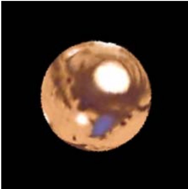
Figure 8. The small North Polar Cap can be seen on the bottom of the image. The large dark albedo feature directly on the central meridian is Syrtis Major. To its south is the large impact region Hellas. Hellas can fill in with fog at times and appear as bright as the polar caps. It is sometimes mistaken for the South Polar Cap.
