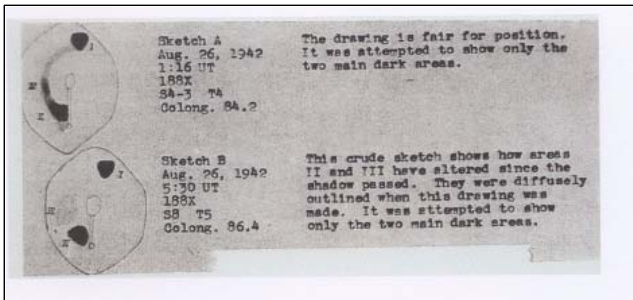
Figure 3. Rough sketches by Walter H. Haas of major dark areas in Atlas during total lunar eclipse of August 26, 1942. 15-cm. reflector. Seeing (S) on scale of 1 to 10 with 10 best. Transparency (T) on scale of 1 to 5 with 5 best.
