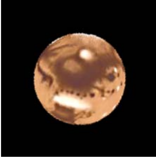
Figure 3: Meridiani Sinus is near the evening limb, with Mare Acidalium directly on the central meridian with white clouds that usually appear in Chryse; these white clouds sometimes appear slightly brighter when a red filter is used, as some dust can get mixed in with the clouds. There are also clouds in Argyre along with some south polar clouds on the top limb. The small North Polar Cap can be seen on the bottom of the image. The Tharsis region is to the right near the morning limb. Solis Lacus is near the southern morning limb.
