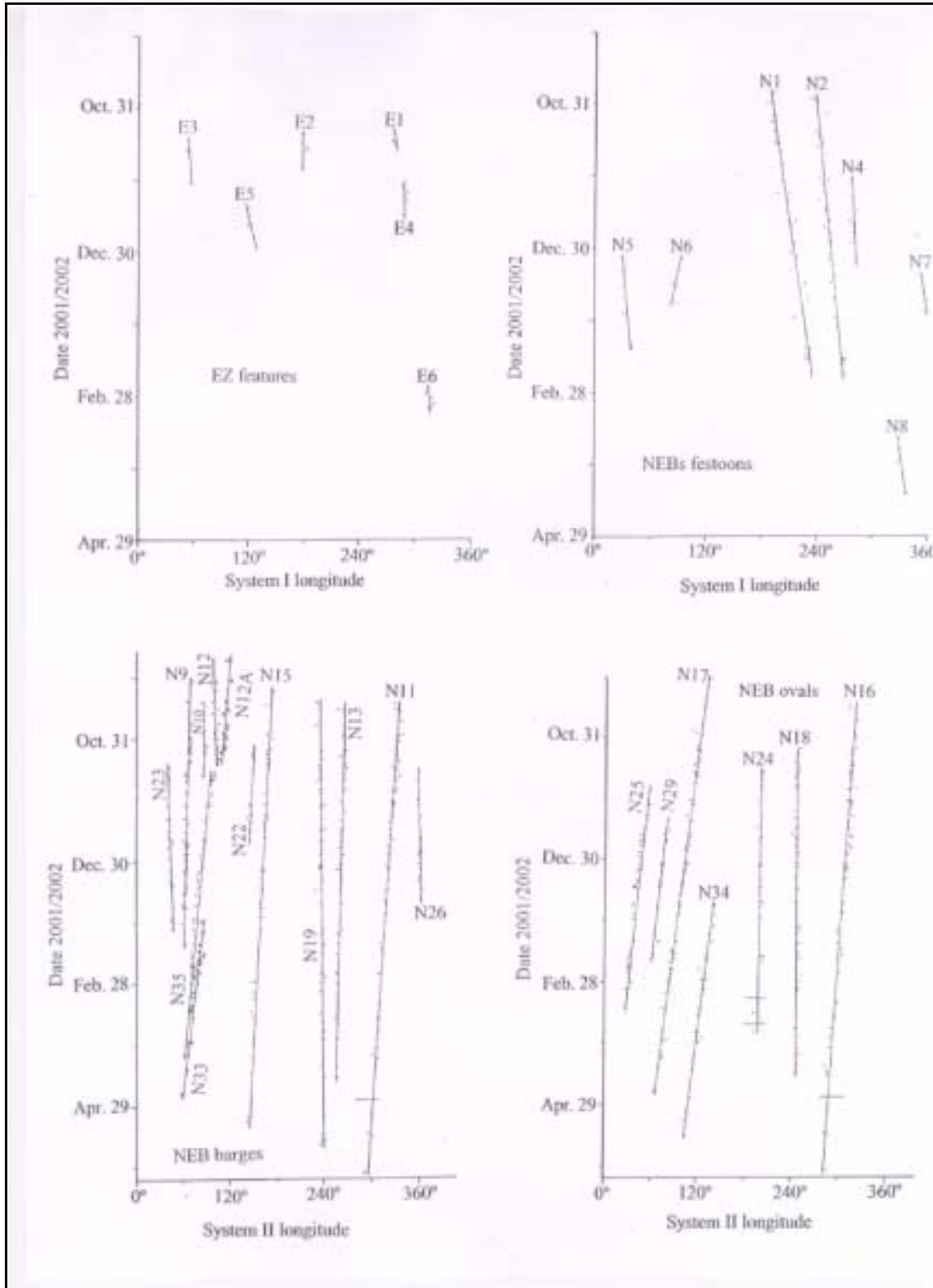
Figure 5: Drift rates of various features in the equatorial zone and in the north equatorial belt. Dots and x's correspond to individual longitude measurements made from CCD images or from central meridian transit times. Horizontal lines are measurements made from drawings and were only used if no CCD images were available.
