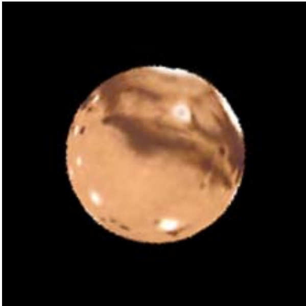
Figure 6: The small North Polar Cap can be seen on the bottom of the image, and the desert region directly on the central meridian is Amazonis. To its left and slightly north is Nix Olympica. Occasionally, this volcano can be seen when it's covered by white clouds. The two very dark features in the south are Mare Sirenum and Mare Cimmerium.
