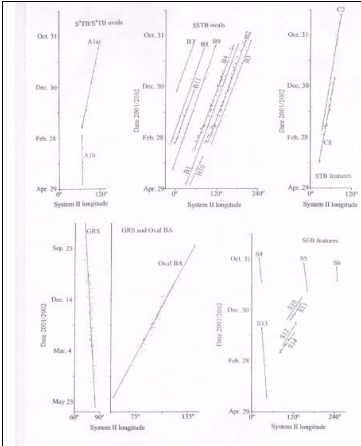
Figure 4: Drift Rates of various features in the southern hemisphere of Jupiter. Dots and x's correspond to longitude measurements.
