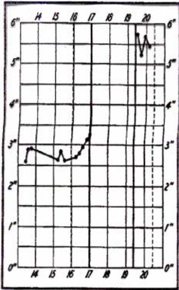
Figure 1. Graph of diameter of Linné White Area during total lunar eclipse of October 16, 1902. Arcseconds vs. Greenwich Mean Time in hours. No measures while in umbra. See also text.
