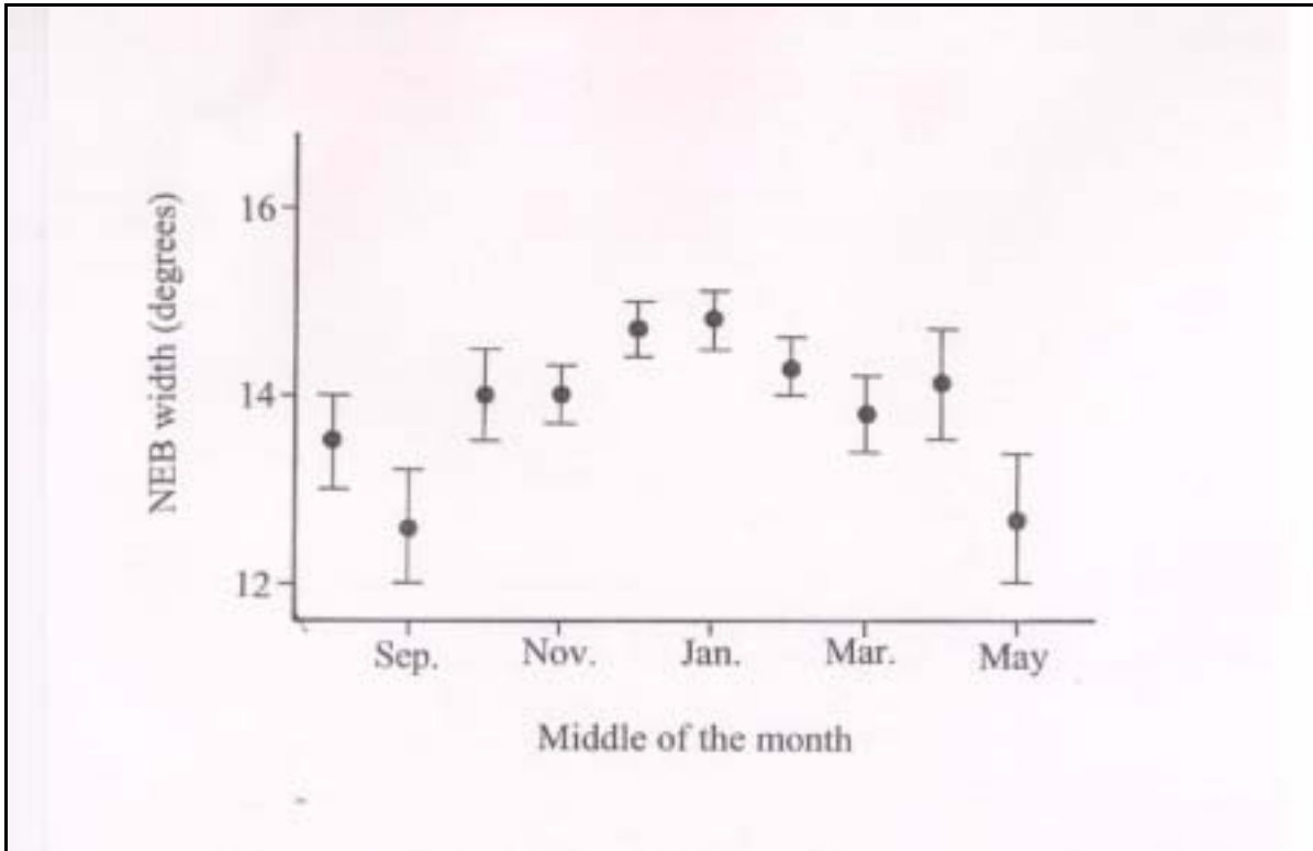
Figure 9: A graph of the width of the North equatorial belt of Jupiter during the 2001-02 apparition.
