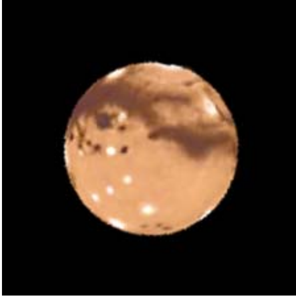
Figure 5: The small North Polar Cap is at the bottom of the image, with the Tharsis region to the left of the central meridian. Solis Lacus is directly on the evening limb in the south with Tithonius Lacus just below it. The large bright white cloud just south of the north polar region is Nix Olympica, while above Nix Olympica is the great Amazonis region.
