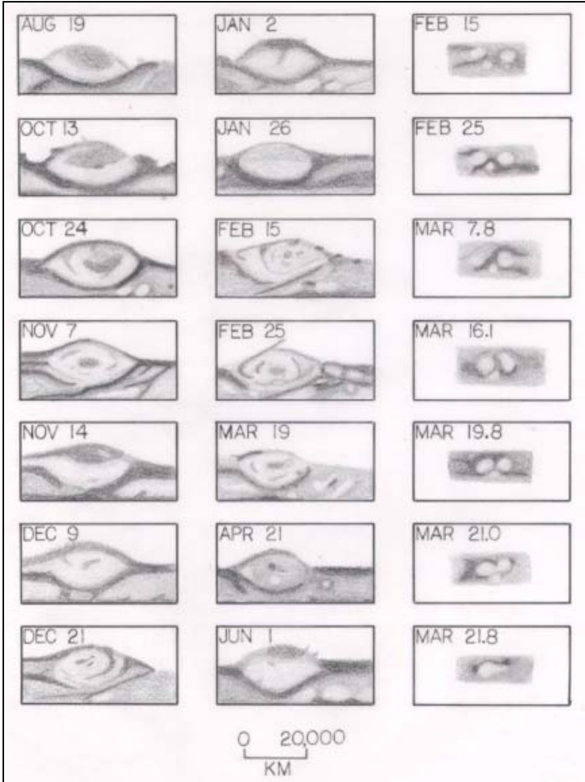
Figure 3: Drawings of the Great Red Spot and the merging of ovals B2 and B3, 2001-2002 Apparition. All drawings were made from CCD images except for the one on Jan. 26, which was made by the author using a 10.2 cm refractor.
