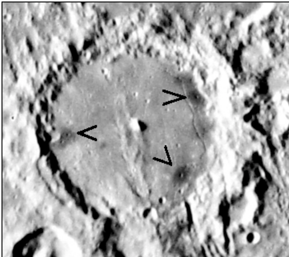
Figure 2: Crater Alphonsus with some of its dark haloed craters marked by arrows. North at top. (From Kuiper, et. al. Consolidated Lunar Atlas . Digital Edition, E. Douglas, E13.
