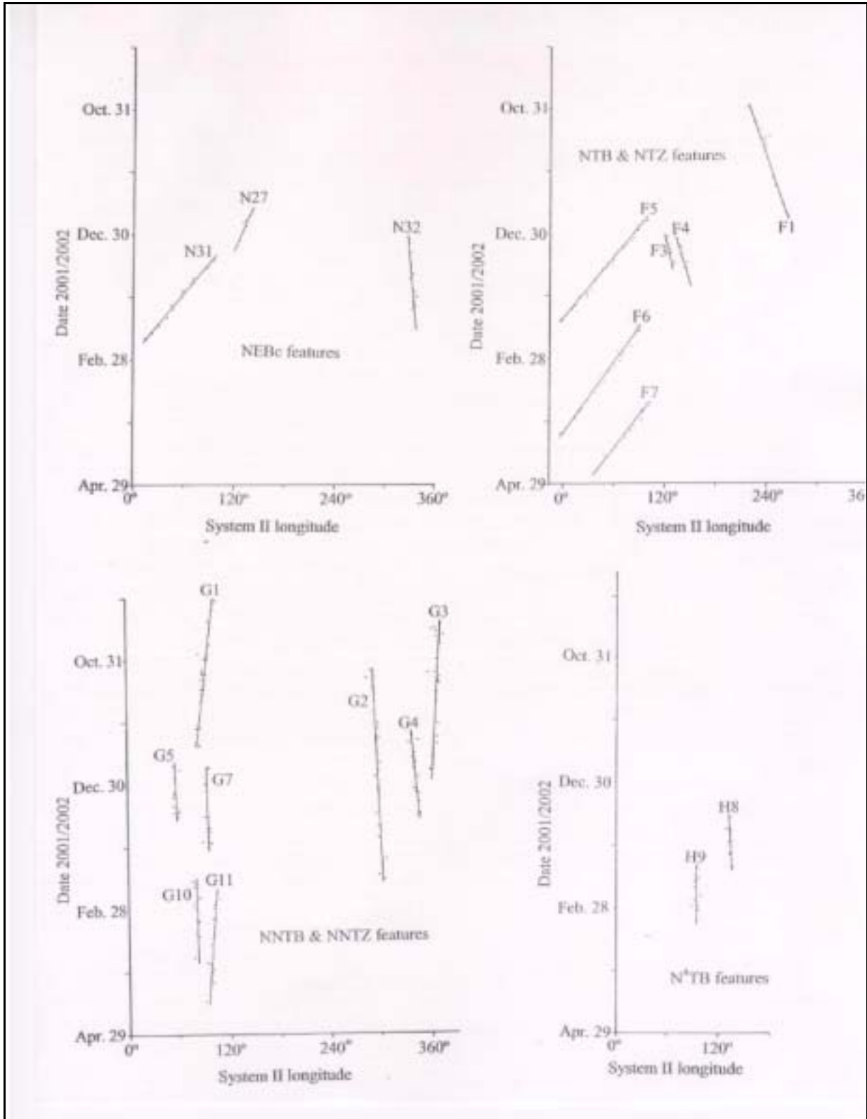
Figure 6: Drift rates of various features in the northern hemisphere of Jupiter. Dots correspond to individual longitude measurements.
