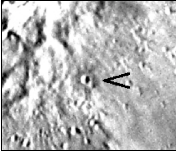
Figure 3: A dark haloed crater southeast of Copernicus. North at top. (From Kuiper, et. al. Consolidated Lunar Atlas . Digital Edition, E. Douglass, D19.
