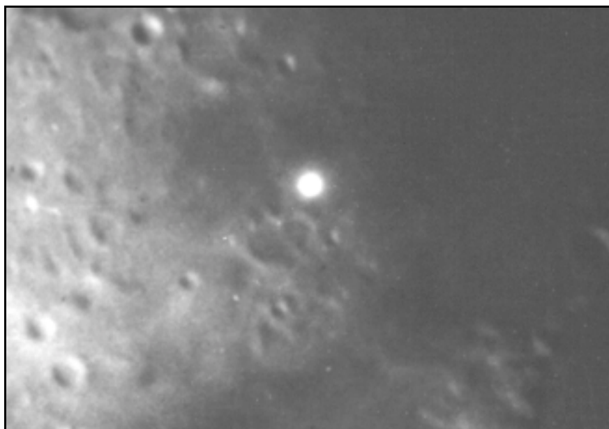
Figure 7. Immediate vicinity of lunar "flare" photographed by Leon H. Stuart on November 15, 1953. Image contributed by Leonard B. Abbey.
