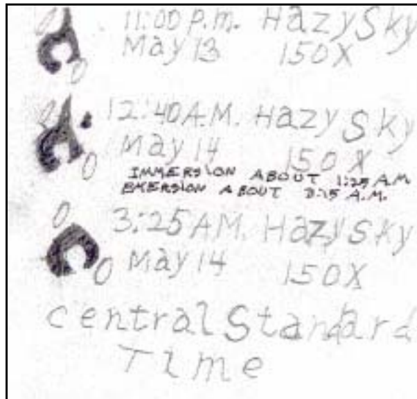
Figure 2. Sketches and notes by Noah W. McLeod of dark area in Riccioli during total lunar eclipse of May 14, 1938. Olcott 5-inch telescope. See also text.
