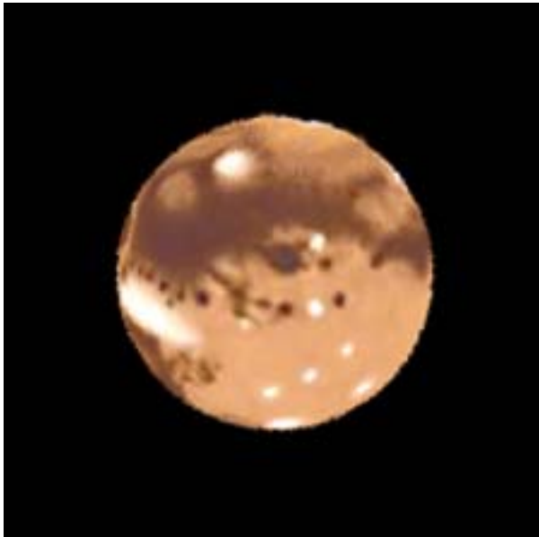
Figure 4: Mare Acidalium is on the evening limb with white clouds that usually appear in Chryse. As stated in Figure 3, these white clouds sometimes appear slightly brighter when a red filter is used as some dust can get mixed in with the clouds. There are also clouds in Argyre along with some south polar clouds on the top limb. The small North Polar Cap can be seen on the bottom of the image. The Tharsis region is seen to the right of the central meridian. Solis Lacus is directly on the central meridian with Tithonus Lacus just below it. The large bright white cloud just south of the north polar region is Nix Olympica.
