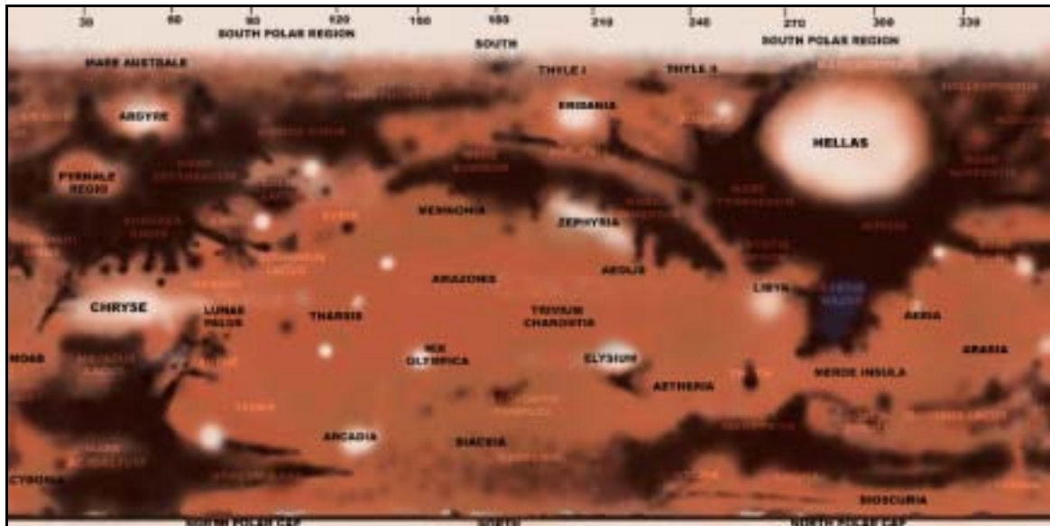
Figure 1: Color version of the 2000-2001 Mars apparition map. South is at top. The white seen over the South Polar Region during most of the observing season is the South Polar Cap. North is at bottom and shows the bright white North Polar Cap as seen close to opposition date displaying the NPC outliers. Most white areas were clouds, with the "Syrtis Blue Cloud" over Syrtis Major at times. Fog was in the Hellas region and Chryse had a mix of white clouds with a little dust. Orographic clouds were observed over great volcanoes in the Tharsis region. This map was produced by the author using the computer program "PhotoStyler". The hues and colors fit the CCD images perfectly. It was produced using all the data (CCD's, drawings, and photos) that were made using the Meade 12-inch LX200 and in June, 2001, the Meade 8-inch LX200 from the Florida Keys. The original black and white surface map took about 45 hours of computer time to produce. The data from the ALPO Mars Section was used to verify all the features in this map.
