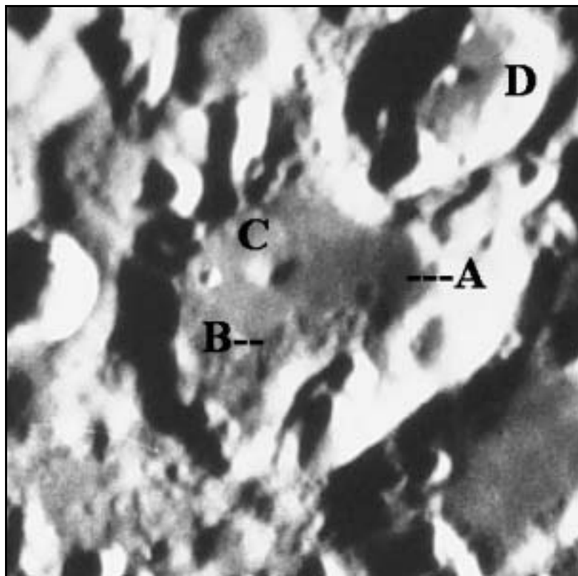
Figure 1: Crater Gemma Frisius, with its cinder cone (A), dark haloed crater (B), and central peak (C). Crater Goodacre (D) overlaps it. North at top. (From Kuiper, et. al. Consolidated Lunar Atlas . Digital Edition, E. Douglass, G12.
