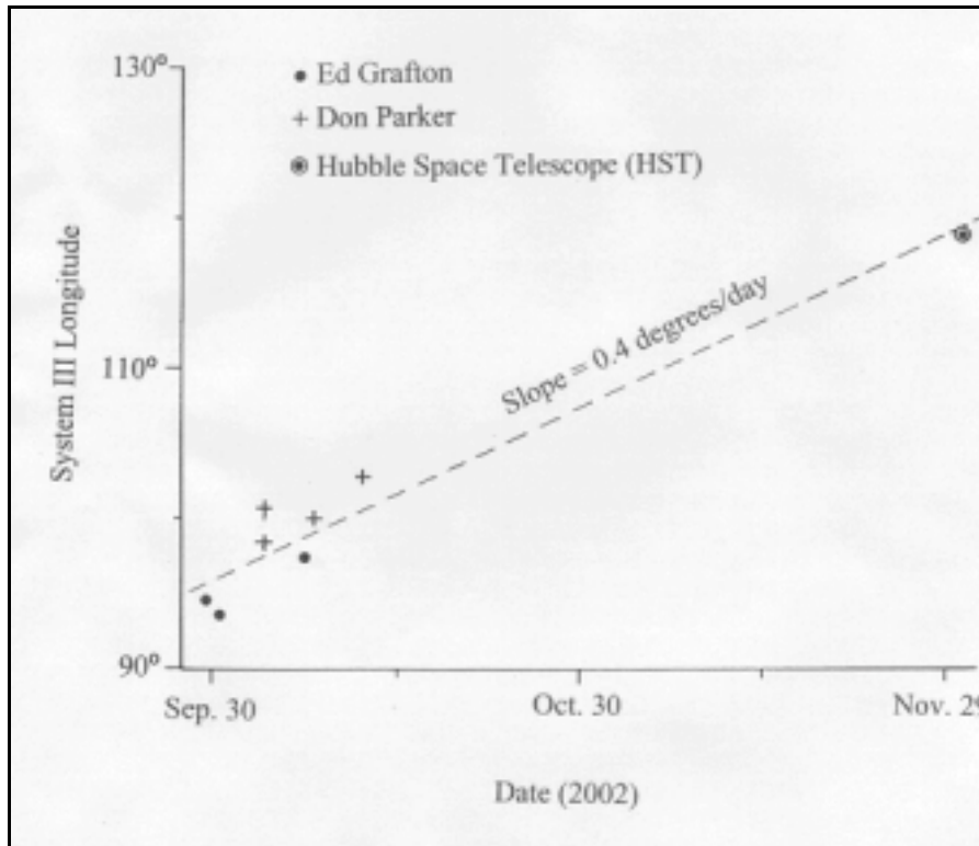
Figure 1: A graph of the longitude of a bright cloud on Saturn plotted against the date. Both amateur and professional data are included in the graph to yield a meaningful slope; the slope is related to the wind speed.. (Ed Grafton and Don Parker are both amateur astronomers.)
