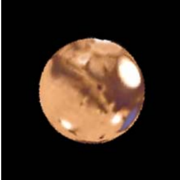
Figure 7: The small North Polar Cap can be seen on the bottom of the image, while just off the central meridian to the left is Elysium, a region that can exhibit white cloud features. Just north of it is the dark feature Aethria, which is a widely variable feature that needs to be watched. Another area that occasionally exhibits white cloud features is Libya, which is right next to Syrtis Major (at right on globe).
